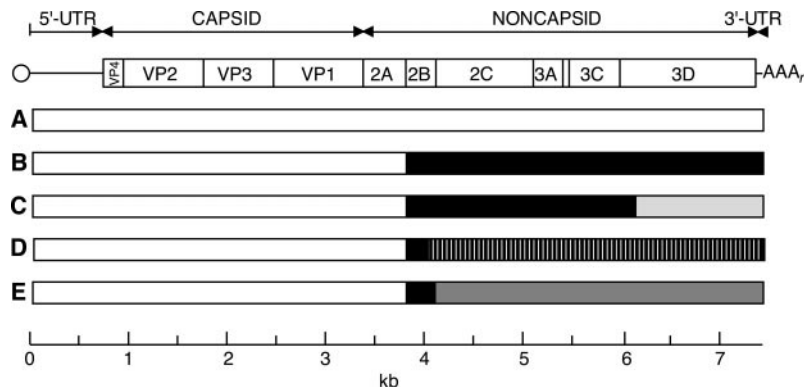
Fig. 4. Location of recombination breakpoints of the four different recombinant classes found among Hispaniola VDPV isolates. In the schematic of the poliovirus genome, the single open reading frame is indicated by a rectangle, flanked by the 5'- and 3'-untranslated regions (UTR). In rectangles A to E, Sabin 1–derived sequences are indicated by white fill, and sequences derived from enteroviruses other than the Sabin OPV strains are indicated by shaded or hatched fills. The rectangles symbolize sequences of A, Sabin 1; B, DOR00-013; C, DOR00-041c1; D, HAI00-003; and E, HAI01-007 (6).
