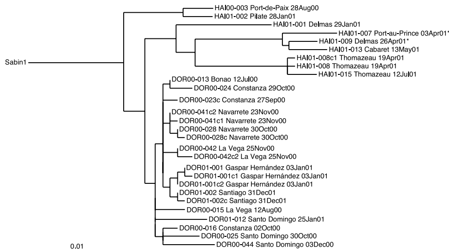
Fig. 3. Maximum likelihood tree (6) of VP1 sequence relationships among the Sabin 1 OPV strain (root of tree) and 28 type 1 VDPV isolates from the 2000–2001 outbreak in the Dominican Republic and Haiti. The location of the case and date of onset of paralysis are shown for each isolate. The isolates from the fatal cases in Haiti (HAI01-007 and HAI01-009) are indicated by asterisks. Isolate pairs that had identical VP1 sequences (DOR00-041c2, DOR00-041c3; DOR00-042, DOR00-042c1; HAI01-008c1, HAI01-008c2) are represented only once on the tree.
